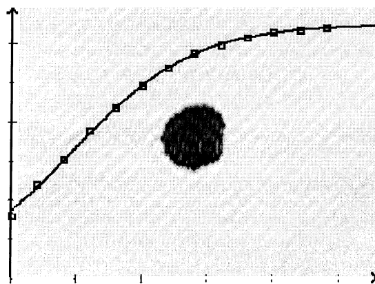
Figure 6 Logistic Growth of a Stain
