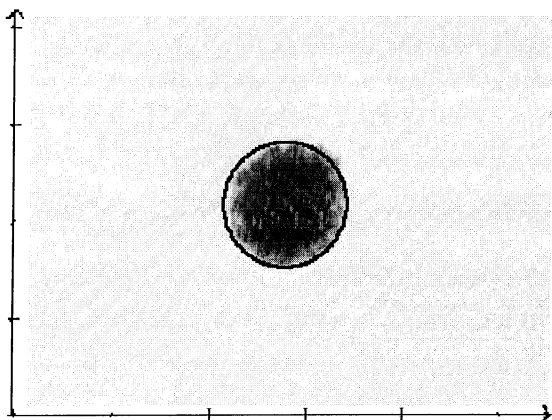
Figure 5 Using the Circle Function
