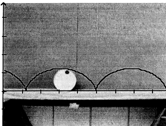
Figure 2 Modeling a Cycloid
