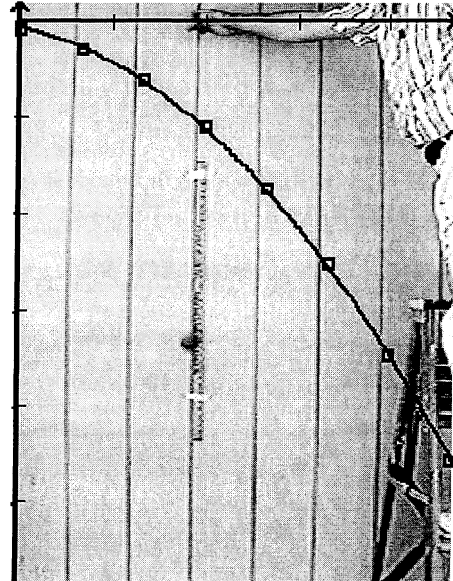
Figure 8 Free Fall Flight of a Ball
