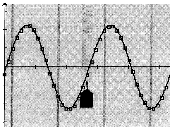
Figure 3 Modeling Periodic Motion
