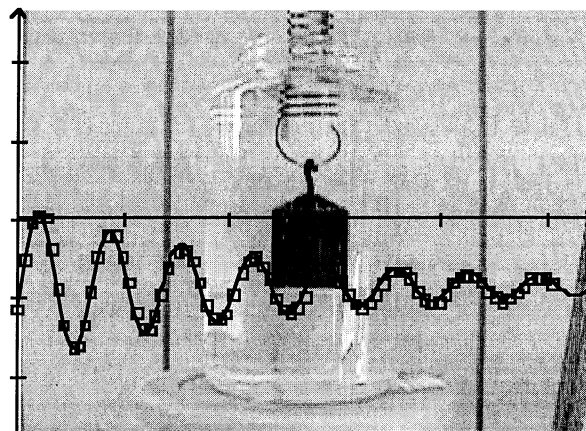
Figure 4 Damped Harmonic Motion
