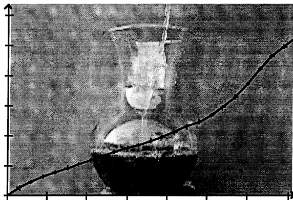
Figure 1 Modeling the Depth of Water
